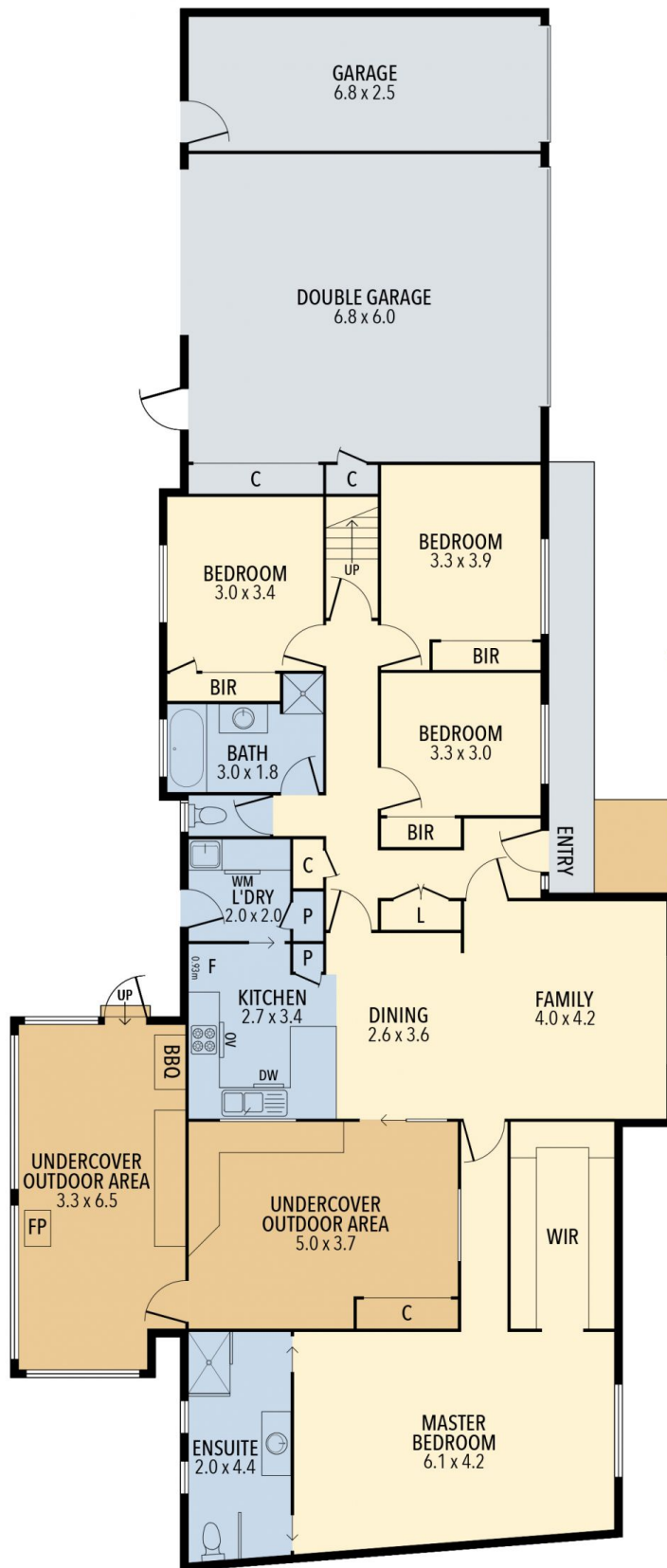
GROUND FLOOR
